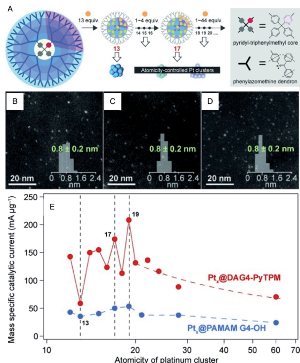
Fig. 7 (A) Illustration of the precise synthesis method of atomically precise Pt NCs using a dendrimer reactor. HAADF-STEM images of (B) Pt 13 , (C) Pt 17 and (D) Pt 19 NCs. (E) Variations of the mass ORR activity vs. the atomicity of the Pt NCs. Panels (a)–(e) are reproduced with permission from ref. 45. Copyright 2015 Wiley-VCH.
