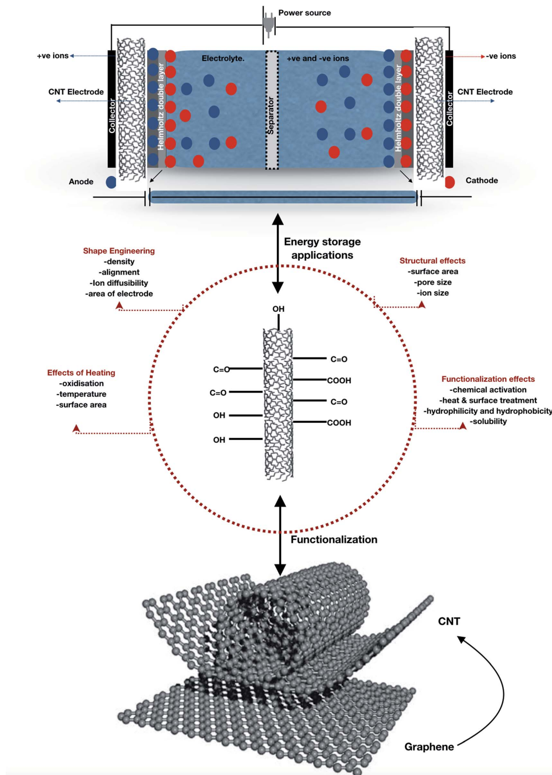
Fig. 13 CNT network for supercapacitor applications and its effects.
