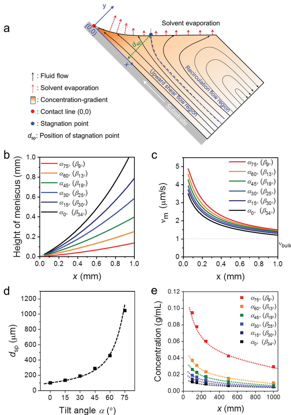
Fig. 3 Fluid simulation for ADDC based on \nu_{bulk}(0^\circ) . (a) Key parameters in the applied meniscus model. (b) Meniscus height for different \beta derived from the optical images in Fig. S1b (ESI † ). (c) Evaporation rate ( v_m ) as a function of x . (d) Position of the stagnation point ( x_{sp} ) as a function of \alpha . (e) Solute concentration at the meniscus ( c_m ) as a function of \alpha .
