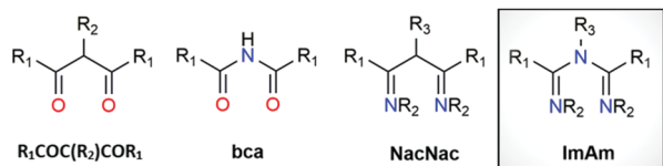
Scheme 1 Structure of 1,3-diketones ( R_1COC(R_2)COR_1 ), bis(carbonyl)amide ( bca ), 1,3-diketoinimate ( NacNac ) and imidoil amidine ( ImAm ).
