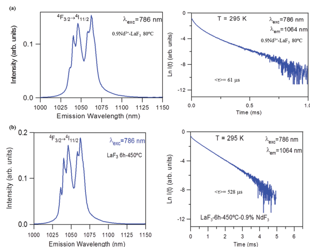
Fig. 8 (a) Emission spectrum of 0.9\text{Nd}^{3+} - \text{LaF}_3 nanoparticles treated at 80^\circ\text{C} and corresponding semi-logarithmic plot of the experimental decay under excitation at 786 nm collecting the luminescence at 1064 nm. (b) Emission spectrum of 0.9\text{Nd}^{3+} - \text{LaF}_3 nanoparticles treated at 450^\circ\text{C} for 6 h obtained under excitation at 786 nm and corresponding semi-logarithmic plot of the experimental decay obtained after excitation at 786 nm collecting the luminescence at 1064 nm.
