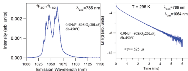
Fig. 9 Emission spectrum of 450 °C–6 h 0.9Nd 3+ –80SiO 2 :20LaF 3 sol and its corresponding semi-logarithmic plot of the experimental decay under excitation at 786 nm collecting the luminescence at 1064 nm.
