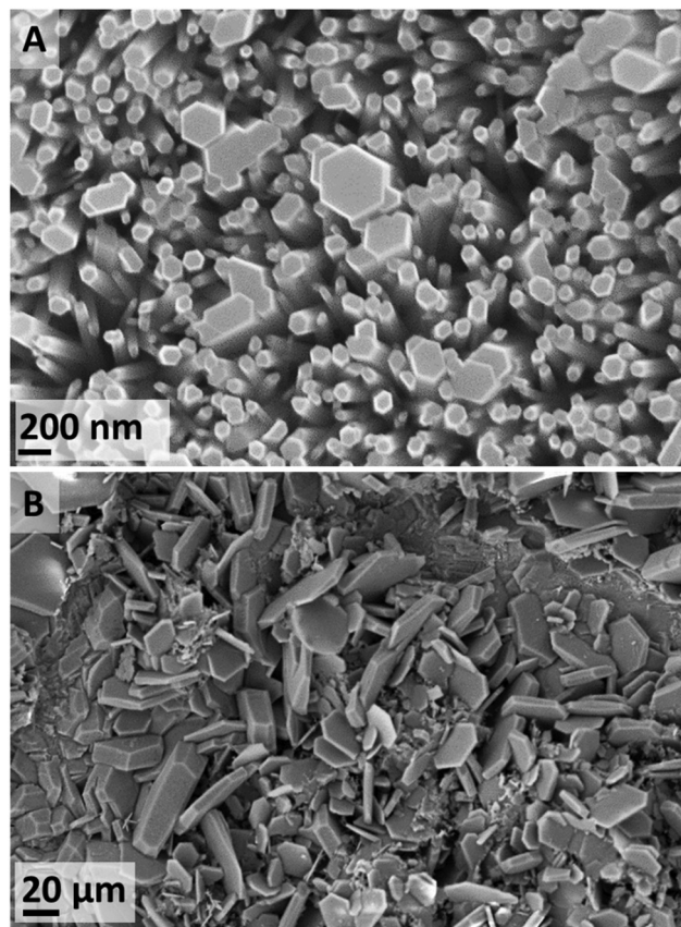
Fig. 4 Magnified zinc surface exposed to [C 4 C 1 im]Cl (IL-1, X_{H_2O} = 0.98 solution at 70 \pm 1 °C). (A) ZnO nanorods after 4 d exposure (magnification 134.17k\times ) (average size 90 \pm 40 nm, n = 361 ). (B) ZHC plate-like crystals after 15 d exposure (magnification 1.44k\times ). Estimated thickness 2.5 \pm 1.5 \mu m ( n = 85 ), diameter 19 \pm 8 \mu m ( n = 85 ).
