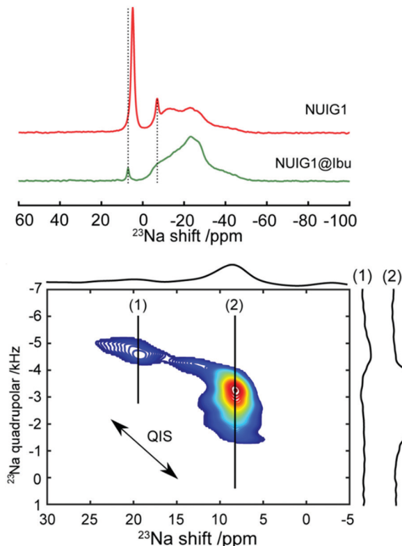
Fig. 6 Top: ^{23}\text{Na} solid-state NMR spectrum of unloaded (red) and loaded (green) MOF. Bottom: DQF-TOP-STMAS ^{23}\text{Na} spectrum of the loaded MOF. Two separate resonances (1) and (2) can be identified. Horizontal extracted slices of these resonances are also represented. The arrow indicates the direction of the second order quadrupolar induced shift (QIS), which accounts for the small differences in resonance position between the one-dimensional spectra (top) and the two-dimensional spectrum (bottom).
