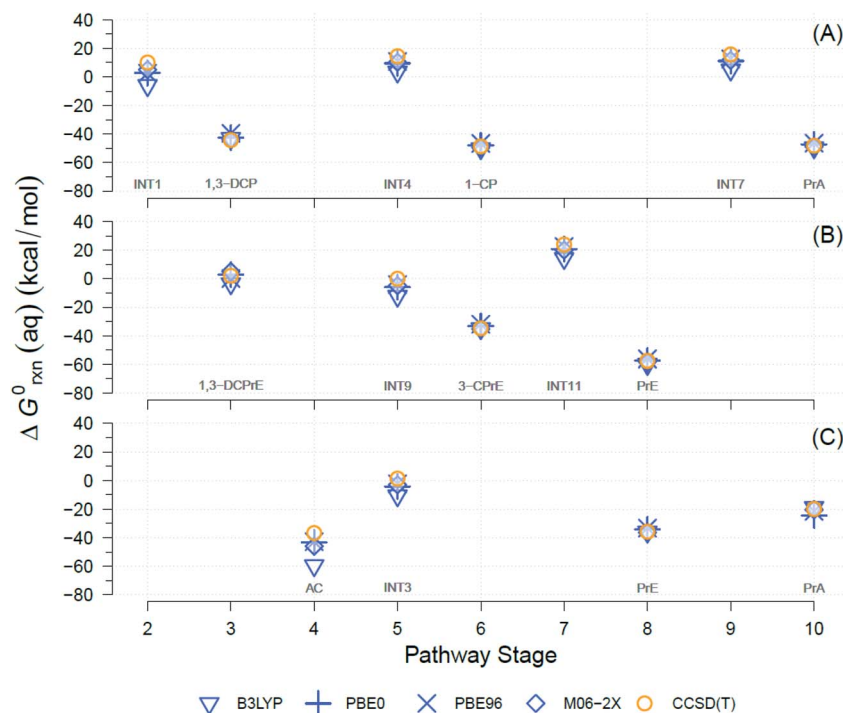
Fig. 3 Comparison between theory levels for computationally derived aqueous phase Gibbs free energies ( \Delta G_{\text{rxn}}^0 (aq), kcal mol -1 ) of individual reactions for selected TCP transformation pathways shown in Fig. 2. Theory levels: DFT, in blue, and CCSD(T), in yellow. Exchange-correlation functionals for DFT: B3LYP, PBE0, PBE96, and M06-2X. (A) Pathway (1): HGL ( trans -branch), (B) pathway (2): DHX ( trans -branch), and (C) pathway (3): BRE + HDG. Pathway stage numbers indicate progression of the transformation route and specifically refer to the reaction coordinate (RC) assigned to the main reaction products (see Sections 3.4 and 3.5 for details). RCs and abbreviations listed and defined in Table S1.† H-atom model used: hydron (H + ) (see Section 3.3 for details).
