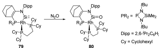
Scheme 29 Oxygenation of the cyclic (amino)(rhodium) silylene 79 by N 2 O.
