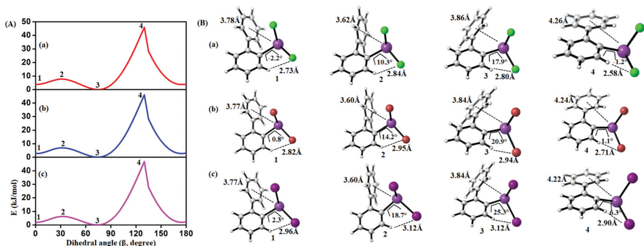
Fig. 18 (A) Computed potential energy surface of halogen ( X ) substituted (2\text{-PhC}_6\text{H}_4)\text{BiX}_2 along with \text{C}-\text{C}-\text{C}-\text{C} dihedral ( \beta ) rotation at PBE-D3/def2-TZVPP level of theory (1 and 3 (2 and 4)) denotes the local minima (maxima) of the respective compound). (B) Selected conformers of (2\text{-PhC}_6\text{H}_4)\text{BiX}_2 taken from PES; (a) X = \text{Cl} , (b) X = \text{Br} , (c) X = \text{I} . Respective dihedral angle, shortest hydrogen bond distance between the nearest hydrogen (H) atom and halogen (X), center-to-center distance between bismuth atoms and phenyl moieties are shown in each geometry. For details on the dihedral definition see ESI.†
