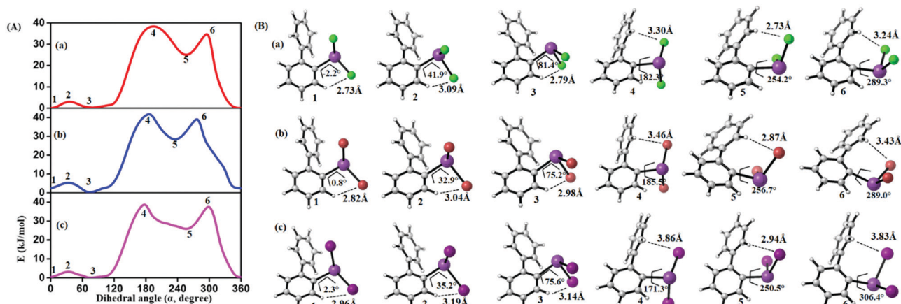
Fig. 17 (A) Computed potential energy surfaces ( (2\text{-PhC}_6\text{H}_4)\text{BiX}_2 ; (a) X = \text{Cl} , (b) X = \text{Br} , (c) X = \text{I} , along with relaxed \text{C}-\text{C}-\text{Bi}-\text{X} dihedral ( \alpha ) scan at PBE-D3/def2-TZVPP level of theory. (B) Selected conformers of (2\text{-PhC}_6\text{H}_4)\text{BiX}_2 taken from PES; (a) X = \text{Cl} , (b) X = \text{Br} , (c) X = \text{I} . The respective dihedral angle and the shortest hydrogen bond between the nearest hydrogen atom and halogen are shown in each geometry (1, 3, and 5 (2, 4, and 6)) denotes the local minima (maxima) of the respective compound). For details on the dihedral definition see ESI.†
