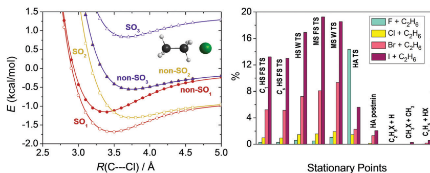
Fig. 5 Potential energy curves obtained at the MRCI+Q(5,3)/aug-cc-pVDZ level as a function of the \text{C}_2\text{H}_6 \cdots \text{Cl C}_{3v} separation (left panel). 12 Deviation in percent between the computed energy difference of the spin-orbit ( \text{SO}_1 ) and non-spin-orbit ( \text{non-SO}_1 ) ground states regarding each stationary points (see Fig. 7 for notations) of the \text{X} + \text{C}_2\text{H}_6 [X = F, Cl, Br, I] reactions and the 1/3 of the experimental SO splitting of the halogen atoms (right panel). 12
