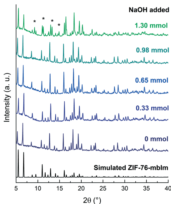
Fig. 4 Powder X-ray diffraction patterns of ZIF-76-mbIm with varying NaOH in the synthesis. Reduction of the number of moles of base used in the synthesis from 1.30 mmol (light green) to 0 mmol (dark blue) systematically improved the purity of the product with 0.65 mmol providing the best combination of purity and yield. Asterisks used to highlight additional peaks in the diffraction pattern.
