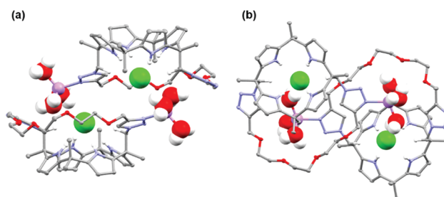
Fig. 2 (a) Side view and (b) top view of the crystal structure of the 2:2:6 complex ( 1 : \text{LiCl} : \text{H}_2\text{O} ). Minor hydrogen atoms and solvent are omitted for clarity (green: \text{Cl} , pink: \text{Li} , red: \text{O} , grey: \text{C} and blue: \text{N} ).
