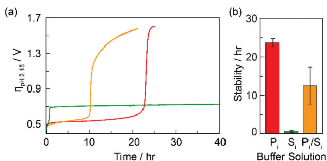
Fig. 2 Stability of \text{CoFePbO}_x films performing OER at 1 \text{ mA cm}^{-2} in buffer solutions ( \text{pH} 2.15 ) of 1 \text{ M KNO}_3 + 0.1 \text{ M KP}_i (red, \text{P}_i ), 1 \text{ M KNO}_3 + 0.1 \text{ M KS}_i (green, \text{S}_i ), or 0.8 \text{ M KNO}_3 + 0.1 \text{ M KP}_i + 0.1 \text{ M KS}_i (orange, \text{P}_i/\text{S}_i ): (a) chronopotentiometry curves, and (b) bar graphs indicating average stability (time required to reach the plateau current). \eta_{\text{pH}2.15} = E_{\text{appl}} - E_{\text{therm}} where E_{\text{therm}} is the thermodynamic potential for water splitting at \text{pH} = 2.15 and E_{\text{appl}} = applied potential.
