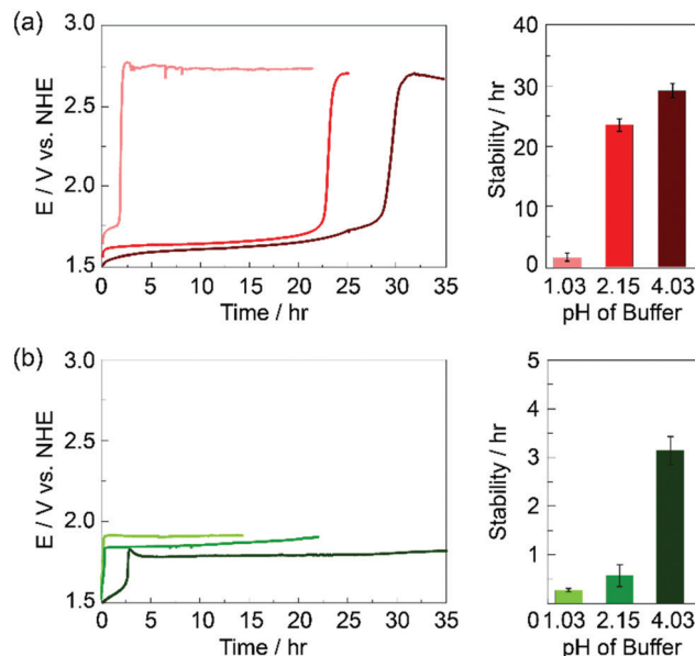
Fig. 3 Stability of \text{CoFePbO}_x films performing OER at 1 \text{ mA cm}^{-2} in solutions containing (a) 1 \text{ M KNO}_3 + 0.1 \text{ M KP}_i and (b) 1 \text{ M KNO}_3 + 0.1 \text{ M KS}_i at different pH: 1.03 (light red and light green), pH 2.15 (red and green), and pH 4.03 (dark red and dark green). Representative chronopotentiometry curves (left), and bar graphs indicating average film stabilities (right) at each pH are shown.
