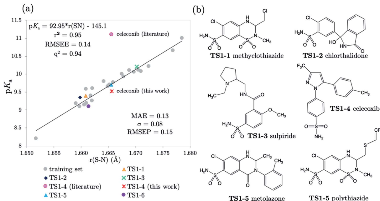
Fig. 3 (a) The relationship between S–N equilibrium bond lengths calculated for the anti -conformer using CPCM and \text{p}K_a values for the 22 Pr-BSA training set compounds, and the equation describing the linear fit; (b) structures of the 6 drug compounds exhibiting a single \text{p}K_a value.
