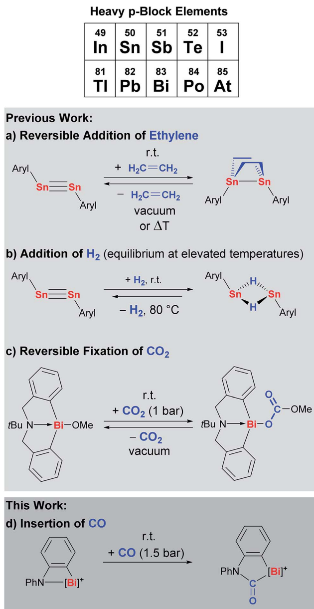
Scheme 1 Examples of well-defined compounds of heavy p-block elements that show unusual reactivity patterns towards small molecules. Aryl = \text{C}_6\text{H}_3\text{-2,6}(\text{C}_6\text{H}_3\text{-2,6-iPr}_2)_2 .
