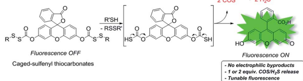
Fig. 1 (a) General design of previous self-immolative COS/H 2 S donors. (b) COS/H 2 S release from fluorogenic caged-sulfenyl thiocarbonate donor motifs.
