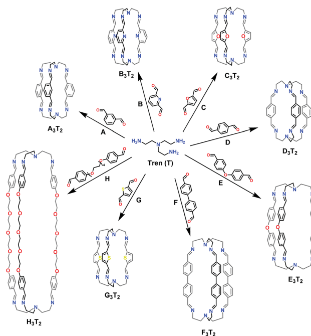
Scheme 1 Molecular structures of dialdehydes ( A–H ), the triamine ( T ) and the generated [3 + 2] homoleptic imine-based organic macrobicyclic cryptand cages.
