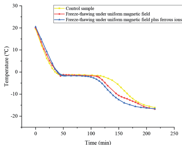
Fig. 1 Influence of uniform magnetic fields on the temperature history of surimi during freezing.
