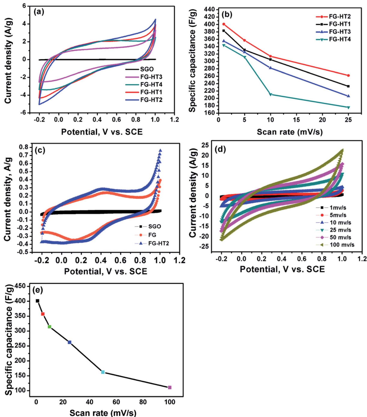
Fig. 6 (a) Comparative cyclic voltammograms of FG-HT1, FG-HT2, FG-HT3 and FG-HT4 nanocomposite at a scan rate of 5 \text{ mV s}^{-1} , (b) average specific capacitances of FG-HT1, FG-HT2, FG-HT3 and FG-HT4 nanocomposites at various scan rates of 1, 5, 10 and 25 \text{ mV s}^{-1} , (c) comparative cyclic voltammograms of FG-HT2, FG and SGO electrodes at a scan rate of 5 \text{ mV s}^{-1} , (d) cyclic voltammograms of FG-HT2 electrodes at different scan rates, and (e) the corresponding specific capacitance of FG-HT2 electrodes at different scan rates in 0.5 \text{ M H}_2\text{SO}_4 .
