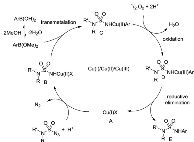
Scheme 5 Possible mechanism.
