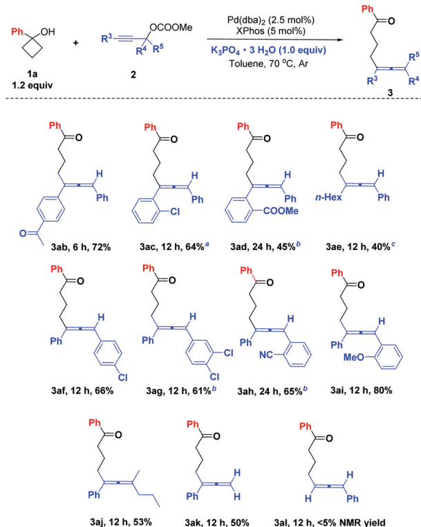
Scheme 5 Substrate scope with respect to propargylic carbonates. Reaction conditions: 1a (1.2 mmol), 2 (1.0 mmol), Pd(dba) 2 (2.5 mol%), XPhos (5.0 mol%), and K 3 PO 4 · 3 H 2 O (1.0 equiv.) in toluene (5.0 mL) at 70 °C. a 1a (1.0 mmol), 2 (1.2 mmol), Pd(dba) 2 (5.0 mol%) and XPhos (10.0 mol%) were used. b Pd(dba) 2 (5.0 mol%) and XPhos (10.0 mol%) were used. c 1a (1.0 mmol) and 2 (1.5 mmol) were used.
