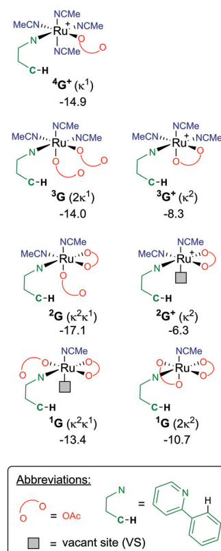
Fig. 9 BP86–D3BJ(BS2,MeCN)//BP86(BS1) free energy values at 120 °C for isomers of G , relative to A , [(C 6 H 5 )Ru(OAc) 2 ], in kcal mol -1 {chemical structures of each isomer do not necessarily represent the most stable intermediate energy quoted, but are to highlight the differences in each “G” species}.
