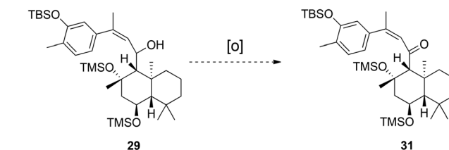
Scheme 6 Attempted oxidation of allylic alcohol 29.
