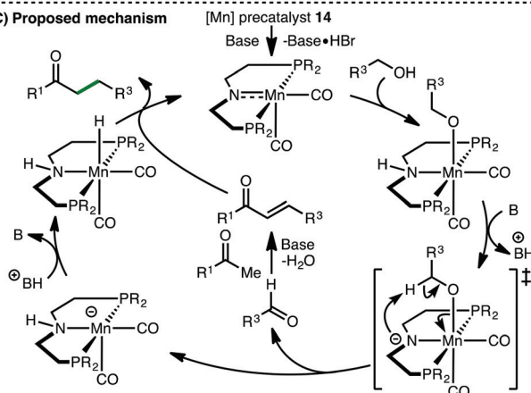
Scheme 24 Mn-Catalysed C -alkylation of ketones and oxindoles (Beller).
