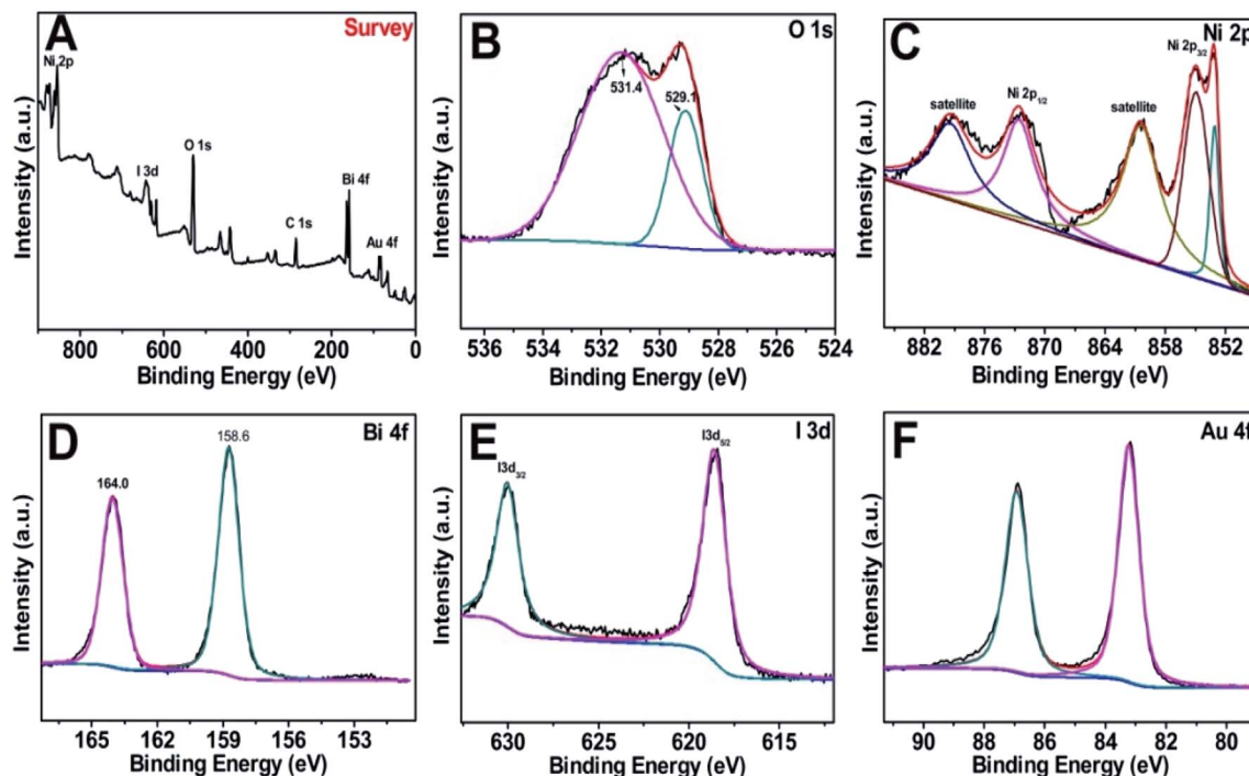
Fig. 3 (A) XPS survey of the as-fabricated Au@BiOI/NiO heterostructure and (B–F) high-resolution XPS spectra of O 1s, Ni 2p, Bi 4f, I 3d and Au 4f, respectively.
