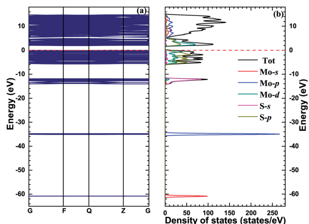
Fig. 2 The band structure (a) and density of states (b) of monolayer \text{MoS}_2 , and the red dashed lines stand for the Fermi level.
