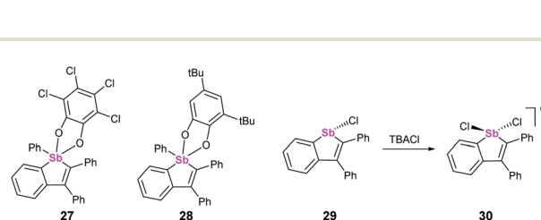
Fig. 9 Structures of stibole-containing systems.
