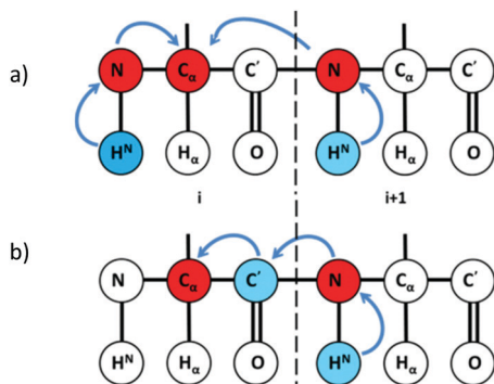
Fig. 1 Magnetization transfer pathway in (a) 2D hNCA providing (C^\alpha_i, N_i) and (C^\alpha_i, N_{i+1}) chemical shift correlations and (b) 2D hNcoCA providing (C^\alpha_i, N_{i+1}) shift correlations.
