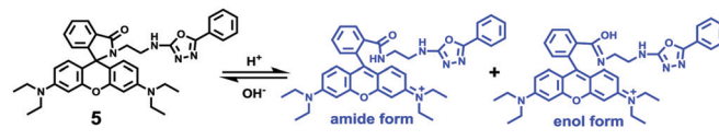
Scheme 5 Fluorescent probe 5 for pH.
