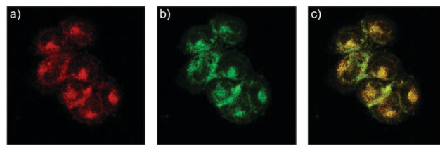
Fig. 8 Fluorescence microscopy images of living HeLa cells co-stained with 1 \mu M probe 4 and 0.25 \mu M LysoSensor green. (a) Red emission from probe 4 ; (b) green emission from LysoSensor green; (c) overlay of (a) and (b); areas of colocalization appear in yellow. Copyright 2014 Elsevier.
