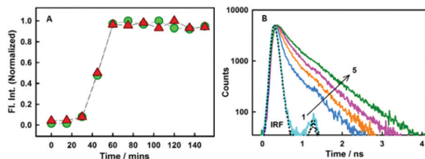
Fig. 3 (A) Normalized plot for the variation in intensity for styryl-11 (triangles) and thioflavin-T (circles). (B) Fluorescence decay traces for 10 \mu\text{M} styryl-11 at various concentrations (in \mu\text{M} ) of insulin fibrils (1) 0 (2) 1.45 (3) 4.2 (4) 7 and (5) 19. The dotted line represents the instrument response function (IRF).
