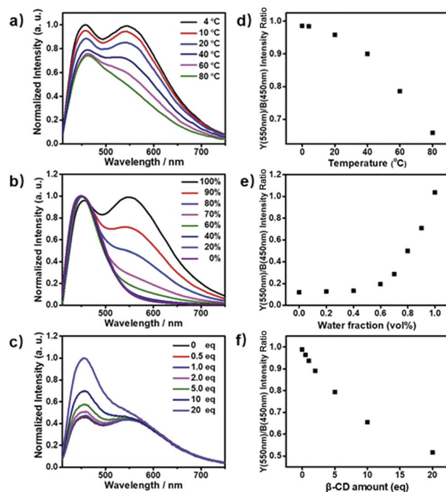
Fig. 5 (a) PL emission spectra of NP4C aqueous solution measured at different temperatures ranging from 4 to 80 ^{\circ}\text{C} ; (b) PL emission spectra of NP4C aqueous solution at different volume fractions of \text{H}_2\text{O} ( f_w , from 0 to 100%) and MeOH, the intensity of the blue light band was unified to the same level; (c) PL emission spectra of NP4C aqueous solution when added with different amounts of the \beta -CD host molecules (from 0 to 20 eq.). The yellow/blue (Y/B) emission intensity ratio as a function of (d) temperature, (e) water fraction f_w and (f) the amount of \beta -CD. All the measurements were taken using aqueous NP4C solutions with a unified concentration ( [\text{NP4C}] = 25 \mu\text{M} ) and excited at 400 nm.
