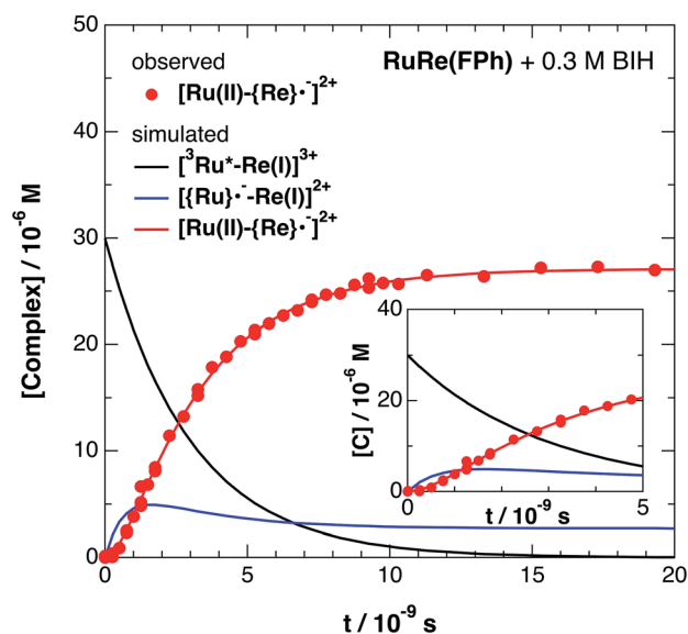
Fig. 7 Time profile of [\text{Ru(II)}-\{\text{Re}\}^\bullet]^{2+} (●) in the ps-TRIR measurement of \text{RuRe(FPh)} in the presence of 0.3 M BIH in an argon-saturated DMF-TEOA (5 : 1 v/v) solution after 532 nm excitation. The kinetic simulation results for [^3\text{Ru}^*-\text{Re(I)}]^{3+} , [\{\text{Ru}\}^\bullet-\text{Re(I)}]^{2+} , and [\text{Ru(II)}-\{\text{Re}\}^\bullet]^{2+} are also shown (solid lines).
