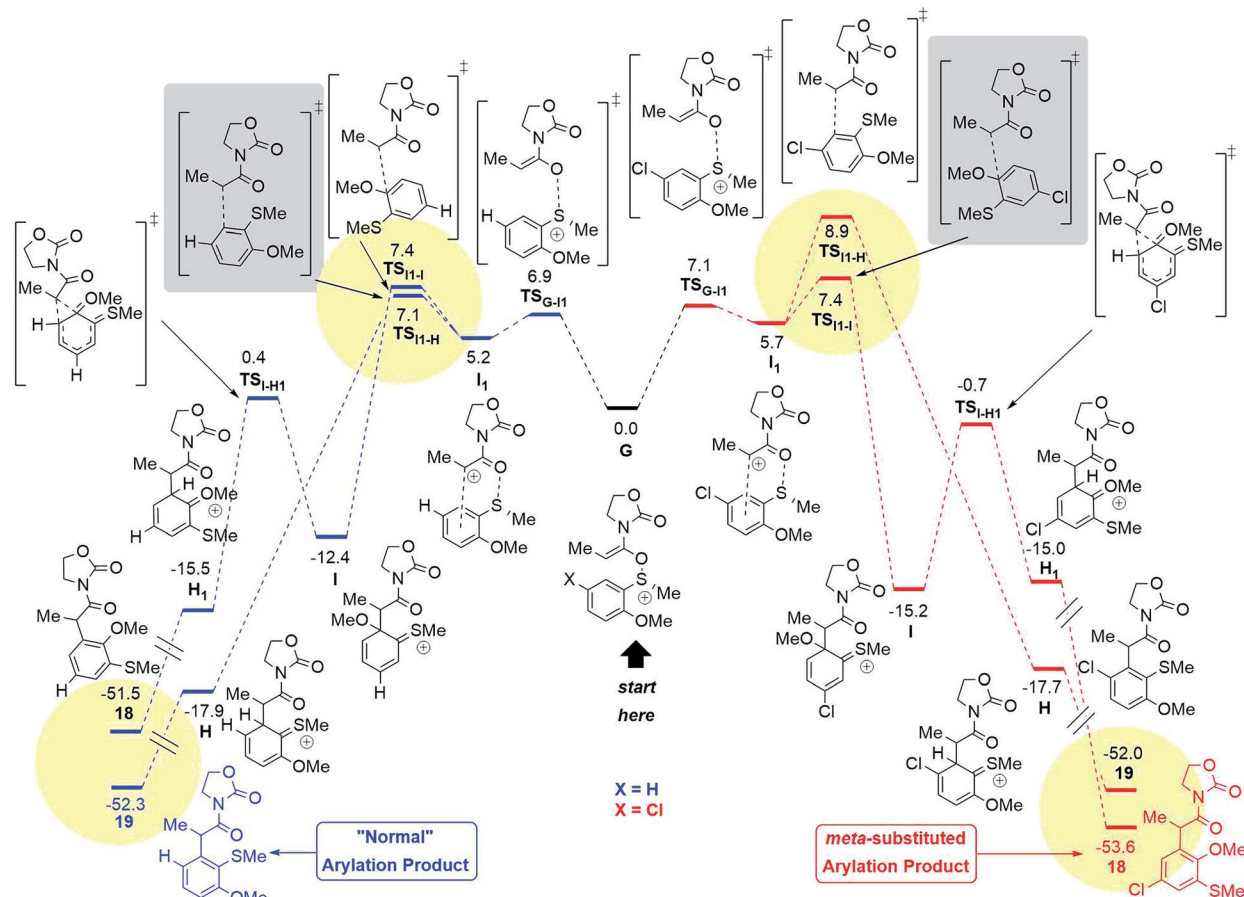
Fig. 10 Computed reaction profile (SCS-R1-MP2-COSMO/def2-QZVP//R1-MP2/def2-TZVP, 24 \Delta G_{298,DCM} ) for the conversion of the intermediate G into both possible products for the X: H (blue) and the X: Cl (red) systems. The summarised energies of the intermediate G and the counterion NTf_2^- are taken as a reference (0.0 kcal mol -1 ). The yellow circles highlight the kinetic and thermodynamic factors, responsible for the regioselectivity. The grey boxes highlight the key transition states responsible for the proposed pathways.
