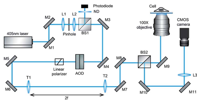
Fig. 2 Schematic of iSCAT microscopy used in our experiments. The beam of a 405 nm diode laser is steered by two AODs for the x and y direction in the sample plane to raster-scan on the target cells inside a glass chamber placed on 100 \times objective [M1–11, mirrors; L1–3, lens; BS1–2, 50 : 50 beam splitters; ND, neutral density filter; AOD, acousto-optic deflector; and T1–2, telecentric lens ( f = 500 mm)].
