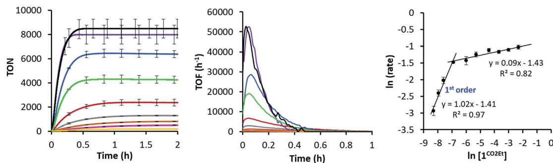
Fig. 5 (Left) Dependence of the \text{H}_2 evolution with the concentration of 1^{\text{CO}_2\text{Et}} (100 \mu\text{M} , yellow; 50 \mu\text{M} , pink; 25 \mu\text{M} , orange; 12.5 \mu\text{M} , grey; 5 \mu\text{M} , red; 2.5 \mu\text{M} , green; 1 \mu\text{M} , blue; 0.5 \mu\text{M} , purple; 0.25 \mu\text{M} , black). (Middle) On-line \text{H}_2 evolved traces and rates vs. time at different concentrations of 1^{\text{CO}_2\text{Et}} (0.25–100 \mu\text{M} ). Conditions: \text{PS}_{\text{Ir}}^+ (150 \mu\text{M} ) in \text{CH}_3\text{CN} : \text{H}_2\text{O} : \text{Et}_3\text{N} (4 : 6 : 0.2 mL) irradiated ( \lambda = 447 \text{ nm} ) at 25^\circ\text{C} . (Right) Logarithmic plot of catalytic rate as a function of 1^{\text{CO}_2\text{Et}} concentration.
