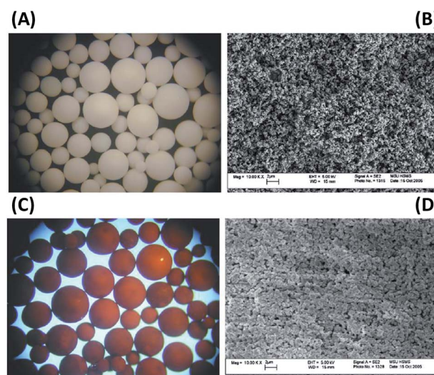
Fig. 6 (A) Light microscope photograph of SBA (45x); (B) SEM images of SBA and (C) light microscope photograph of HFO/SBA adsorbent (45x); (D) SEM images of HFO/SBA adsorbent. 169
