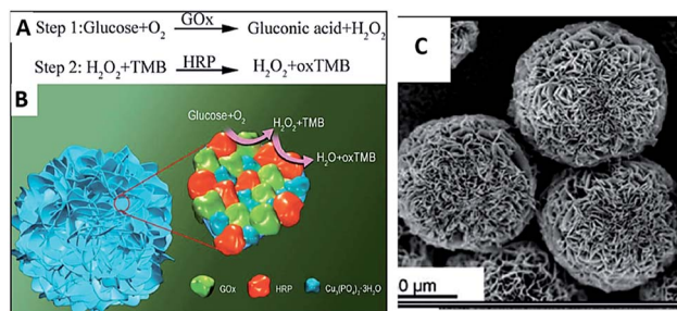
Fig. 2 (A) Proposed mechanism of glucose detection using a two-step enzymatic reaction in one pot. (B) The mechanistic illustration of glucose detection with GOx and HRP and Cu(II)-incorporated nano-flowers. (C) SEM images of GOx and HRP nano-flowers.
