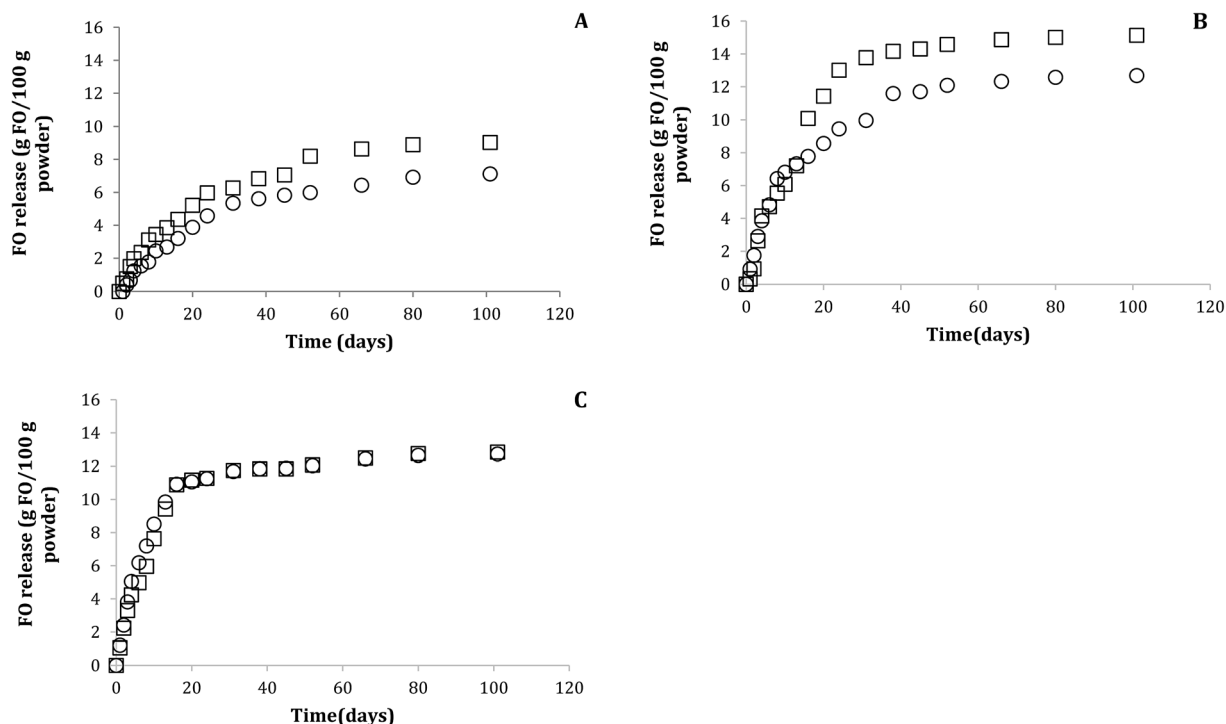
Fig. 3 FO release profile from FO microparticles obtained under optimal conditions (FO-EtOH-Lec (A), FO-EtOH (B) and FO-W-Lec (C), in aqueous models ( \circ pH 4.6, \square pH 6.5) at 30 °C.
