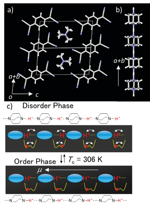
Fig. 3 Dynamic short-range collective proton transfer and dielectric switching in the organic semiconductor (HDABCO ^+ ) 2 (TCNQ) 3 . (a) Unit cell viewed along the 1D (N–H ^+ \cdots N) _{\infty} hydrogen-bonding chain and electrical conducting \pi -column of TCNQ. (b) High temperature 1D (N–H ^+ \cdots N) _{\infty} hydrogen-bonding chain of HDABCO ^+ cations along the a + b axis. Schematic potential energy curves of the N–H ^+ \cdots N hydrogen-bonding chain (c) at the high temperature paraelectric disordered phase (upper) and at the low temperature ordered ferroelectric phase (lower) for the proton orientation.
