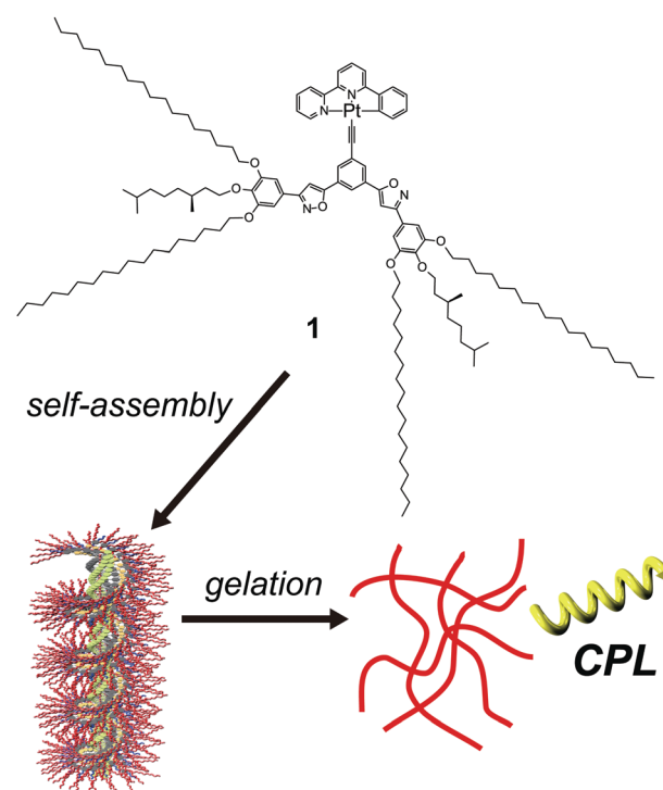
Fig. 1 Schematic representation of the self-assembly and CPL-active organogel of 1 .
