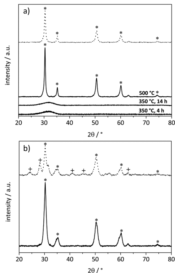
Fig. 1 XRD patterns of (a) the \text{Ag}/\text{ZrO}_2\text{-cp} and (b) the \text{Ag}/\text{ZrO}_2\text{-fsp} catalysts. Solid lines correspond to calcined catalysts and dotted lines represent reduced catalysts ( 350^\circ\text{C} , 2 h, 3 \text{ L min}^{-1} , 10% \text{H}_2 in \text{N}_2 ); *cubic \text{ZrO}_2 , +monoclinic \text{ZrO}_2 .
