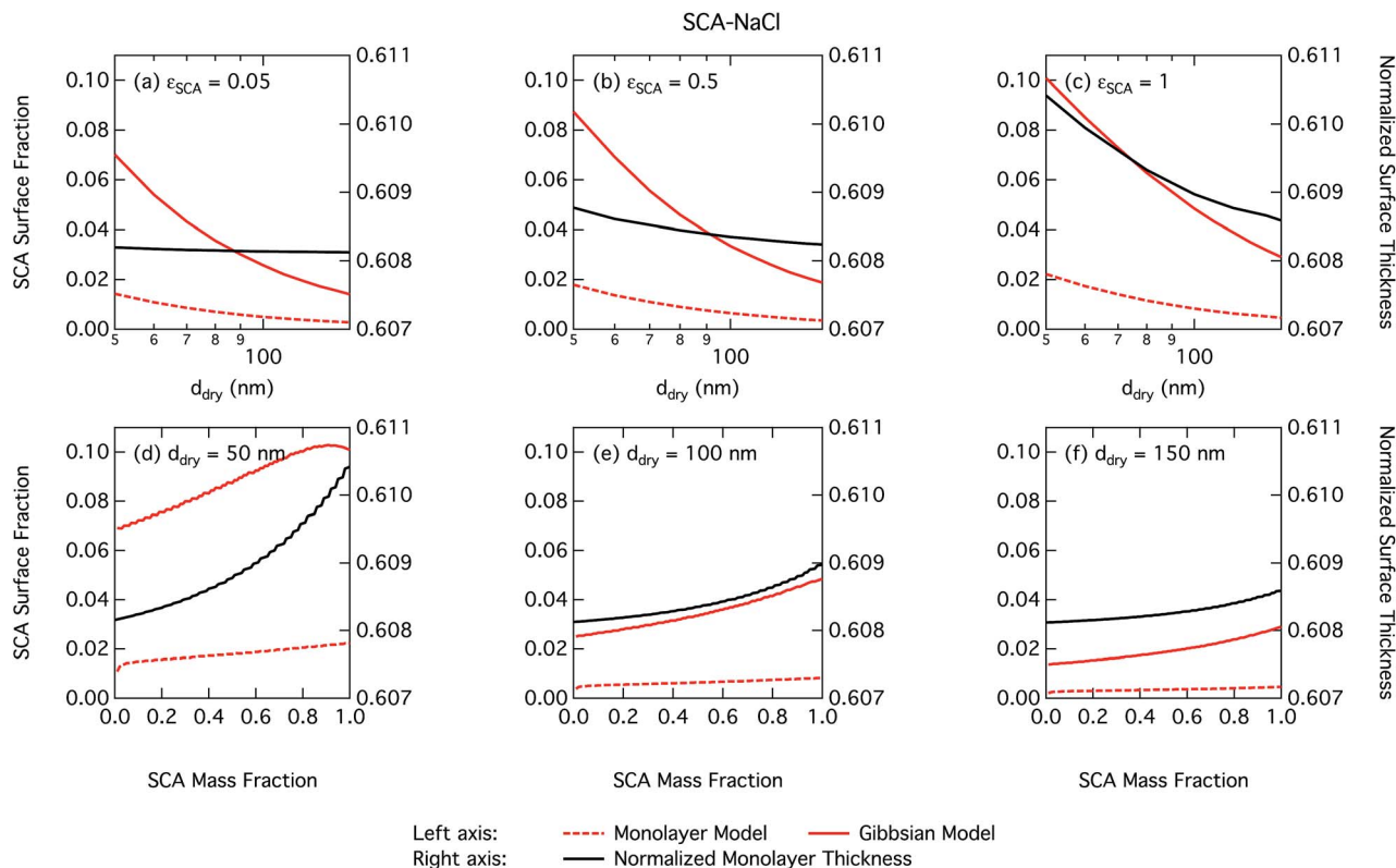
Fig. 4 Droplet SCA surface fraction on the left axes calculated with the monolayer and Gibbs models and surface thickness from the monolayer model normalized to the thickness of one SCA monolayer on the right axes, as a function of dry particle size for SCA mass fractions (a) 0.05; (b) 0.5; (c) 1 and as a function of SCA mass fraction for dry particle sizes (d) 50 nm; (e) 100 nm; and (f) 150 nm.
