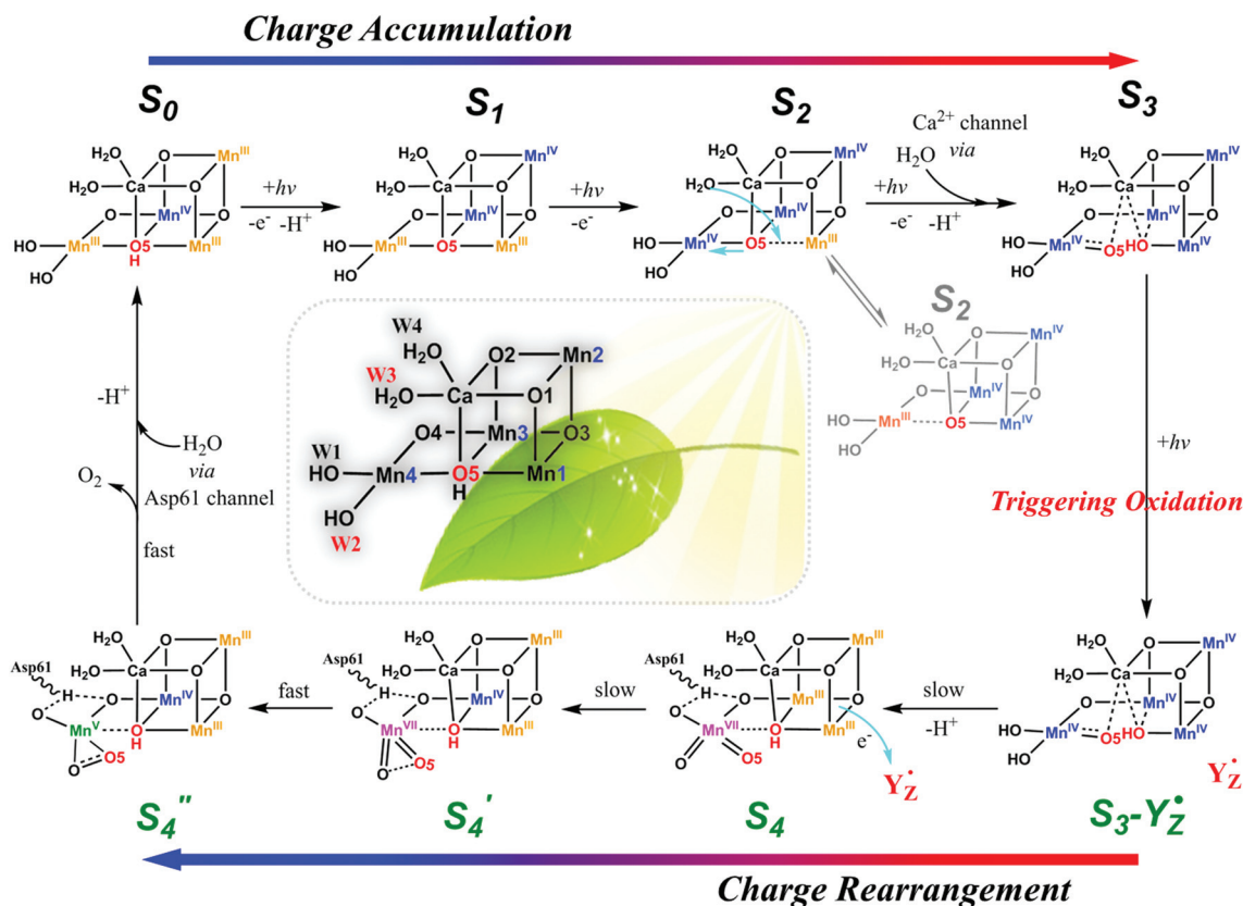
Fig. 2 Proposed catalytic mechanism for water oxidation by \text{Mn}_4\text{CaO}_5 cluster in PSII involving \text{Mn}^{\text{VII}}\text{-dioxo} species. Charge disproportionation of \text{Mn}_4\text{CaO}_5 cluster at the S_3\text{-}Y_Z^* state after accumulation of three charges, i.e., charge rearrangement, leads to the formation of a super-active S_4' [III, III, IV, VII] state after the S_3 \rightarrow S_4 step. An O–O bond forms within the \text{Mn}^{\text{VII}}\text{-dioxo} site (between W2 and O5) during the S_4 \rightarrow S_4' step. W2, O5, and W3 all participate in \text{O}_2 evolution.
