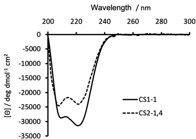
Fig. 2 CD spectra of 30 \mu\text{M} CS1-1 (solid line) and CS2-1,4 (dashed line) peptide monomer, recorded at 293 K in 5 mM HEPES buffer pH 7.0.
