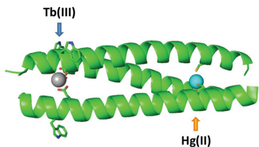
Fig. 1 Cartoon representation showing our designed hetero bimetallic coiled coil, featuring \text{LnAsp}_3 and \text{HgCys}_3 sites towards the N- and C-termini, respectively. Shown are the main chain atoms represented as helical ribbons (green), the Asp, Trp and Cys side chains in stick form (oxygen in red, nitrogen in blue and sulfur in orange), and the metal ions as spheres (lanthanide in grey and mercury in cyan).
