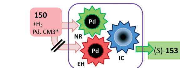
Scheme 45 Cascade nitro group reduction (NR), EH and IC over cinchonidine modified Pd catalyst. 202
