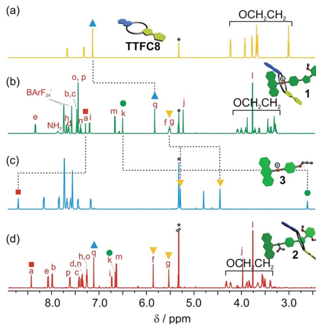
Fig. 3 Stacked partial 1 H NMR spectra (700 MHz, 2 mM, CD 2 Cl 2 , 298 K) of (a) macrocycle TTF C8, (b) charged [2]rotaxane 1 , (c) axle 3 , (d) neutral, acetylated [2]rotaxane 2 . Selected signals are marked with coloured symbols. The solvent residue signal is marked with an asterisk.
