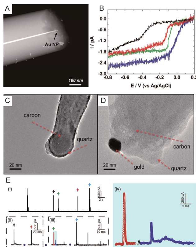
Fig. 4 (A) TEM image of a single Au nanoparticle immobilized on a Pt nanoelectrode. 48 (B) Cyclic voltammetry of a bare 7 nm diameter Pt nanoelectrode (black), a 14 nm Au single nanoparticle immobilized Pt nanoelectrode (SNPE), an 18 nm Au SNPE (green) and a 24 nm Au SNPE (blue) in an oxygen-saturated 0.10 M KOH solution. 48 TEM images of (C) a carbon nanopipette electrode and (D) a carbon nanopipette electrode with a 20 nm AuNP attached to its tip. 93 (E) The current transients of 80 nm collisions of individual AgNPs with a nominal diameter on the Au UME (diameter of UME: 12.5 \mu m) at an applied potential of +0.6 V vs. Ag/AgCl QRE. 73 (i) i - t transients response; (ii and iii) close-ups of the representative spike clusters shown by crosses with different colours. (iv) Enlarged sections of the red and blue transient in (iii). Adapted with permission from ref. 48 Copyright (2010) American Chemical Society. Reproduced from ref. 93 with permission from the Royal Society of Chemistry. Adapted with permission from ref. 73.
