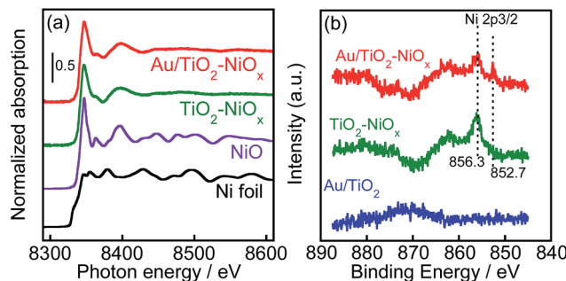
Fig. 4 (a) Ni K-edge XANES spectra of Ni foil, NiO, TiO 2 -NiO x (0.5) and Au(1.0)/TiO 2 -NiO x (0.5); (b) XPS spectra of Au(1.0)/TiO 2 , TiO 2 -NiO x (0.5) and Au(1.0)/TiO 2 -NiO x (0.5) around Ni 2p components.
