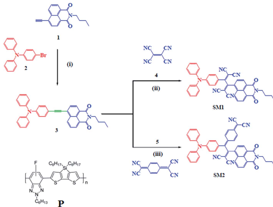
Scheme 1 Synthesis of triphenylamine-substituted 1,8-naphthalimides SM1 and SM2 . Reaction conditions: (i) PdCl 2 (PPh 3 ) 2 , CuI, THF : TEA (1 : 1), 70 °C, 15 h; (ii) CH 2 Cl 2 , 40 °C, 20 h. (iii) C 2 H 4 Cl 2 , 100 °C, 48 h. The chemical structure of the D–A conjugated polymer is also shown.
